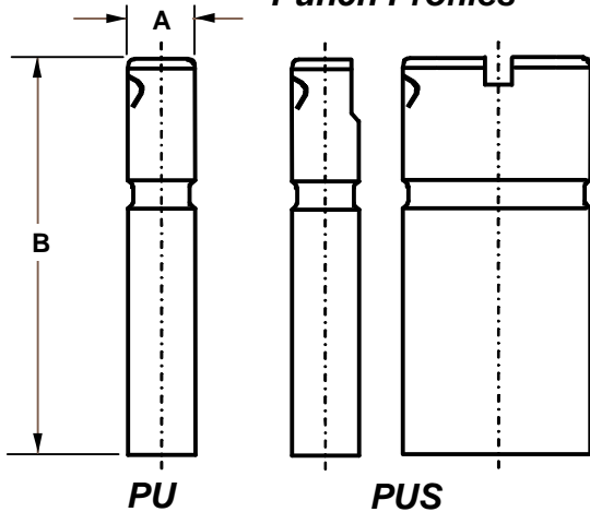
Punch Profiles
